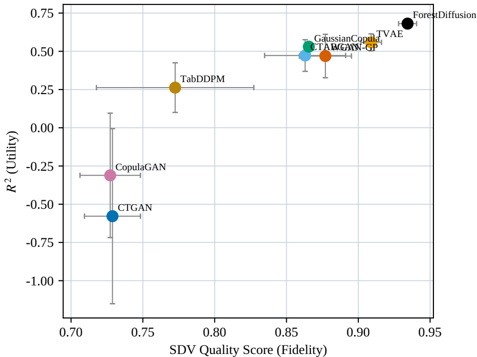
Real Estate: SDV Quality Score (Fidelity) vs R^2 (Utility)
